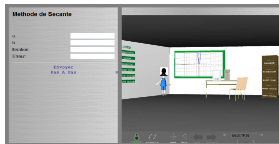
FIGURE 16 TESTING THE SECANT METHOD
