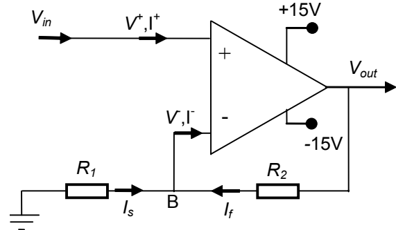
Figure 6 – Non-inverting op-amp circuit
