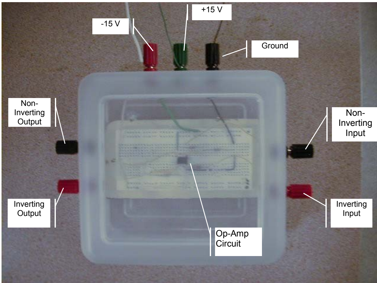
Figure 9 – Op-amp functional module
