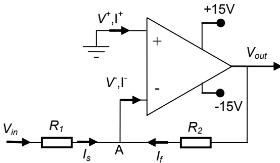
Figure 5 – Inverting op-amp circuit
