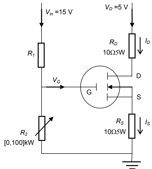
Figure 11 – Field effect transistor circuitry
