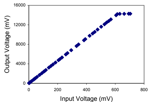
Figure 8 – Non-inverting op-amp output voltage
