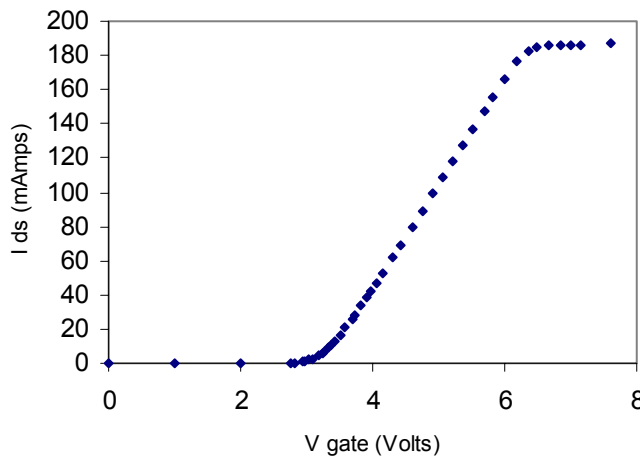
Figure 12 – IRF 530 MOSFET experimental data
